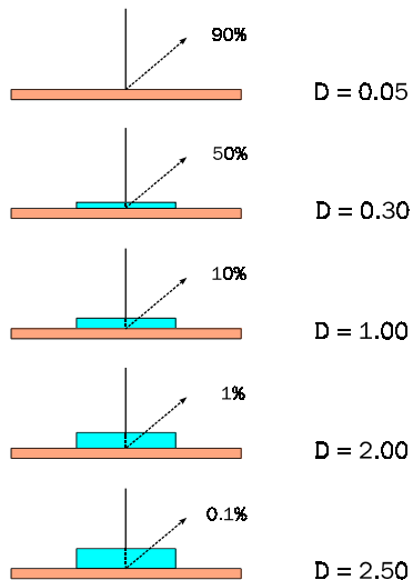
Figure 2: Ink Film Thickness vs. Density
